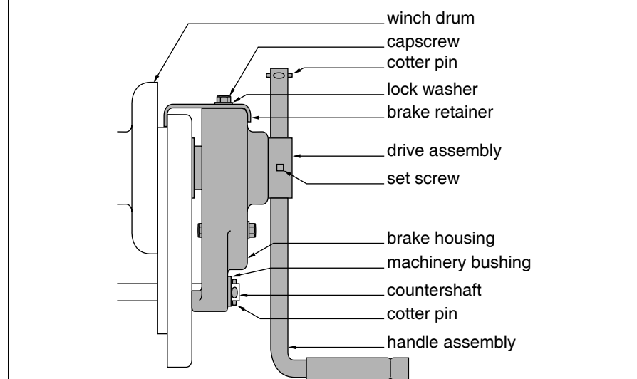
Figure 2 – Model MB441 Installation
