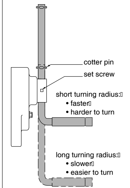
Figure 1 – Adjusting Brake Handle Length
